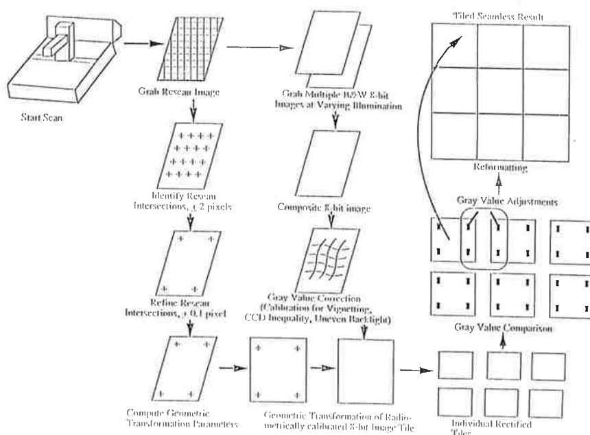
Figure 2: Flow of digitizing process implemented in the VX3000 precision film scanner.
