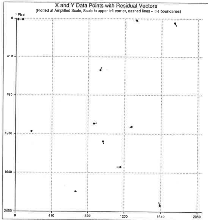
Figure 4: Geometric accuracy plot, obtained by manually measuring 10 randomly located points on a 2050 x 2050 pixel area. Pointing was to the nearest pixel only (no sub-pixel pointing). R.M.S. differences between known coordinates coordinates measured on the scanned image are \pm 0.4 pixels.
