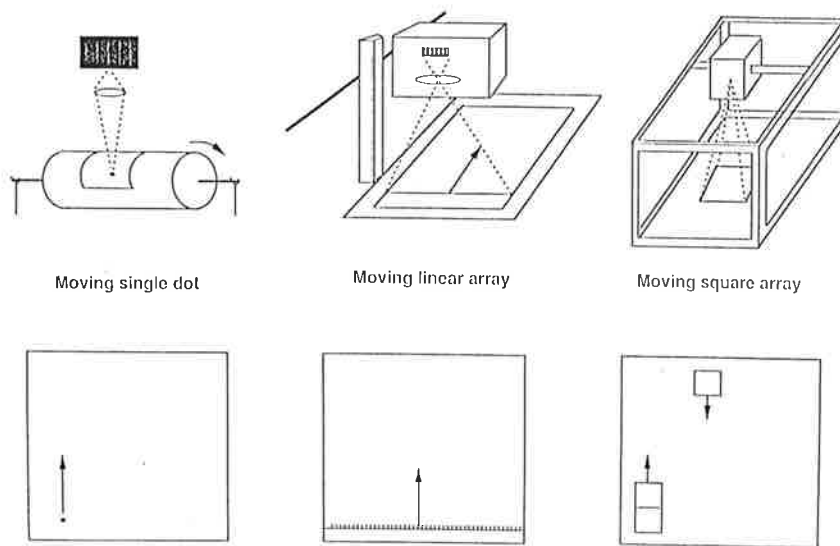
Figure 1: Major scanning technologies using photo-detectors, linear CCD arrays and square array CCDs.
