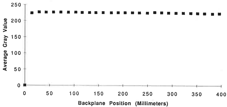
Figure 5: Mean radiometric value observed by the VX3000 of a uniform object at various locations on the film carrier. Ordinate: Digital Number (DN); Abscissa: Millimeters along the backplane. R.M.S. variation is \pm 1.5 DN.
