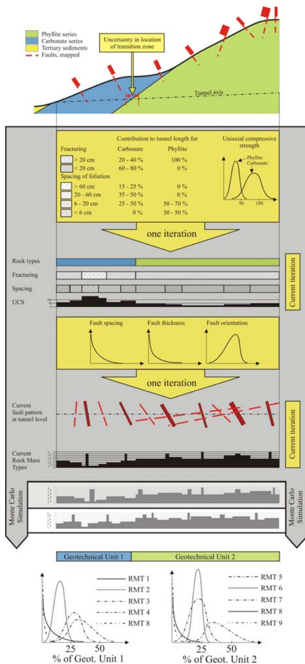
Figure 3. Example for the probabilistic determination of Rock Mass Types
