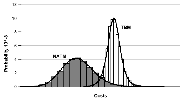
Figure 4. Typical distributions of construction costs for different construction methods
