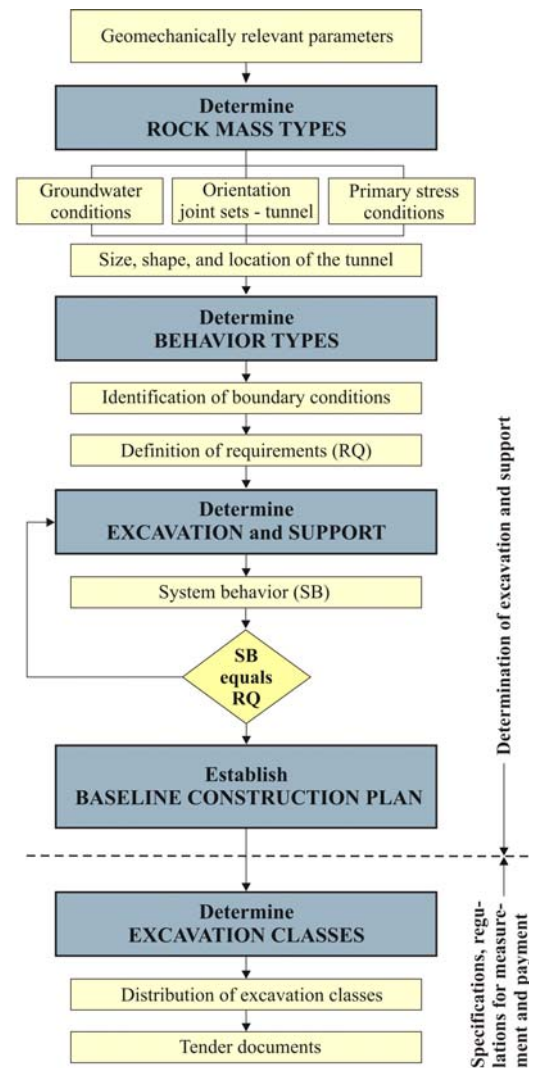
Figure 1. Flow chart of the basic procedure of excavation and support design for underground structures
