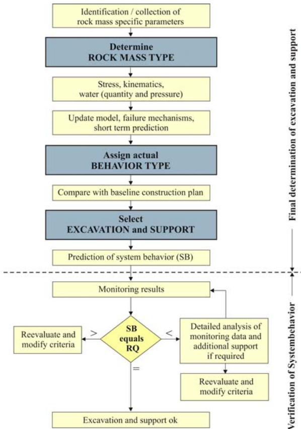
Figure 2. Flow chart of basic procedure during construction
