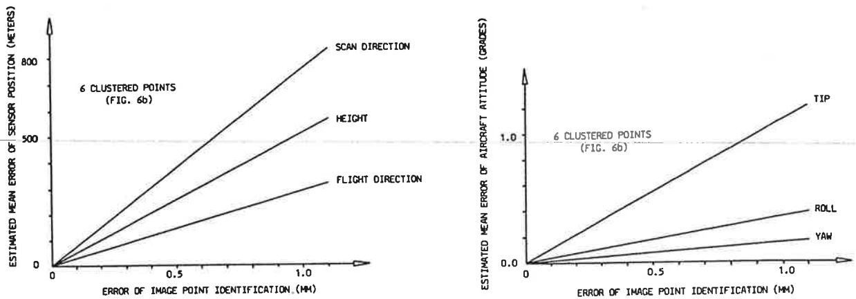
Figure 8: Image identification accuracy versus accuracy of reconstructing aircraft flight position and altitude with the ground control points of Figure 6. Flight height 15,000m above ground, scan angle 0° to 30°, 72" focal length.
