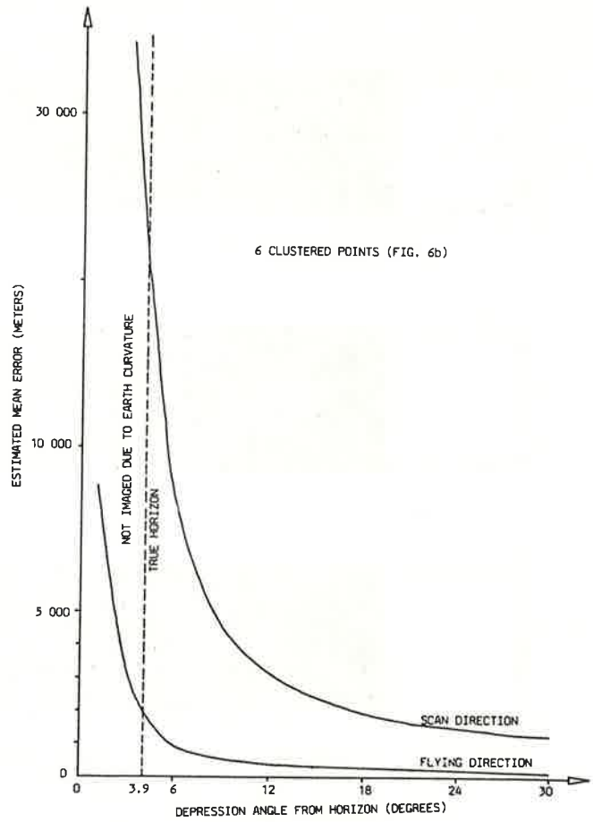
Figure 7: Image identification accuracy versus target position accuracy with the ground control points of Figure 6. Flight height 15,000 m above ground, scan angle of 0° to 30°, 72" focal length.
