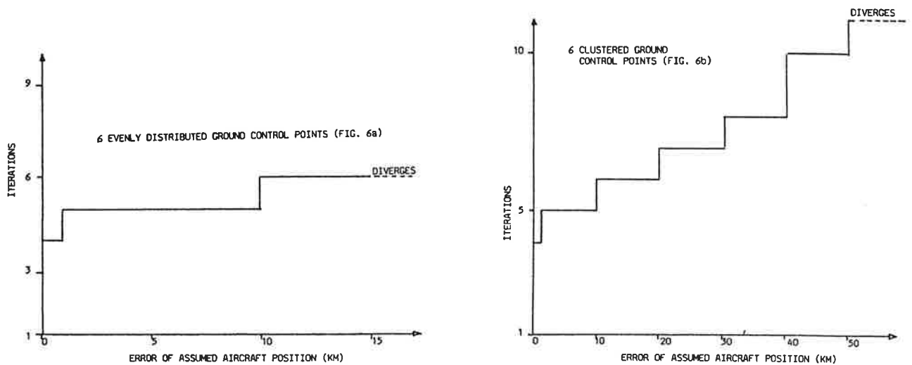
Figure 9: Computational iterations versus errors of approximate aircraft positions; same assumptions as in Figure 7.
