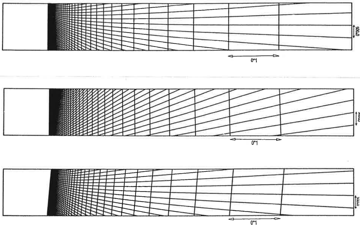
Figure 5: Sector scan panoramic geometry demonstrated by a grid of meridians and parallels, using a scan angle of 0^\circ to 30^\circ from a flight altitude of 15 kms above the ground and a 72" focal length; (a) no attitude errors of the camera; (b) with an aircraft yaw angle of 5^\circ ; (c) with an aircraft tip angle of 5^\circ .
