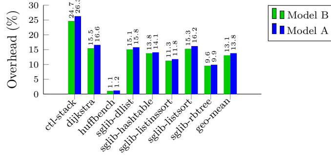
Figure 4.10: Runtime overhead of additional heap interleaving.
