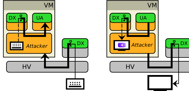
Figure 3.5: Virtualization of driver enclave DX can break the authenticity of secure input (left) and the confidentiality of secure output (right).
