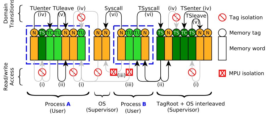
Figure 4.2: Security domains are interleaved in flat physical memory. Tag isolation protects T-domains while MPU isolation encapsulates and protects individual processes across domains. T-domains can only be entered at trusted callable entry points (TC-tag), which allows fast domain transitions.
