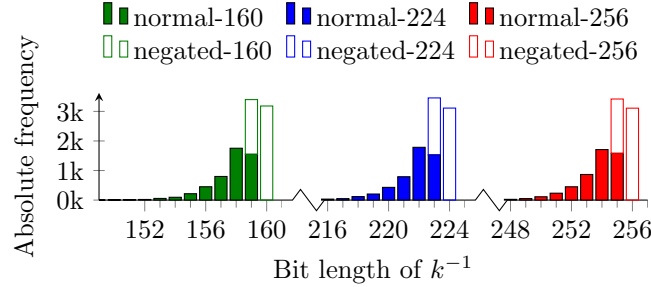
Figure 9.5: OpenSSL DSA leaks the topmost bit of the inverse nonce after Euclidean inversion (V9).
