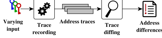
Figure 8.1: Differential address trace analysis searches for differences in recorded address traces.
