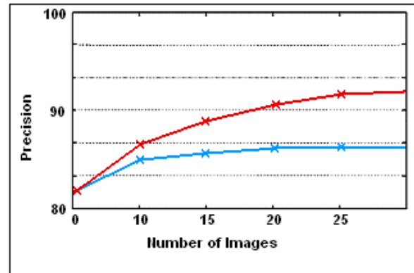
Figure 7: The relationship between the number of images in the multi-view scenario and the precision of window detection (compared in a hand-labelled, rectified façade). The blue line is for the method a) (first merging, then detection), the red line is for the method b) (first detection, then merging).
