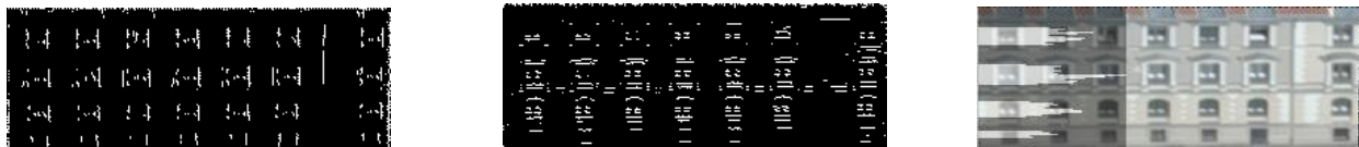
Figure 7, Binary Prewitt edges in (a) are vertical, in (b) horizontal. The sums of edge values are shown in (c) as a count of the number of floors.
