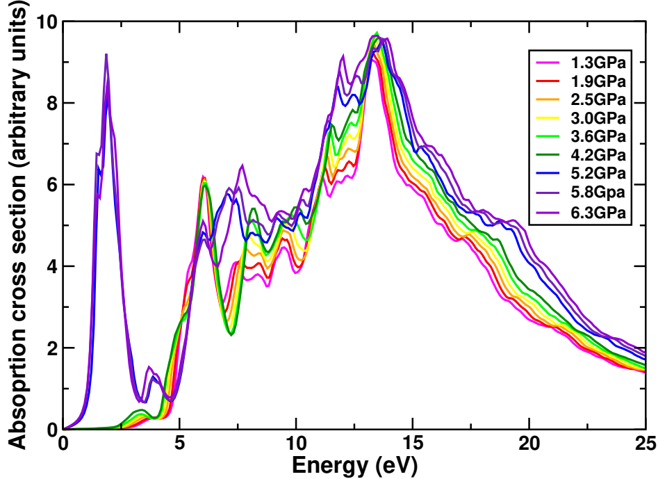
Figure 4: Optical absorption spectra for DMAMnF across the pressure-driven spin transition. The disappearance of the prominent peak around 2 eV absorption energy in the HS state is clearly visible.
