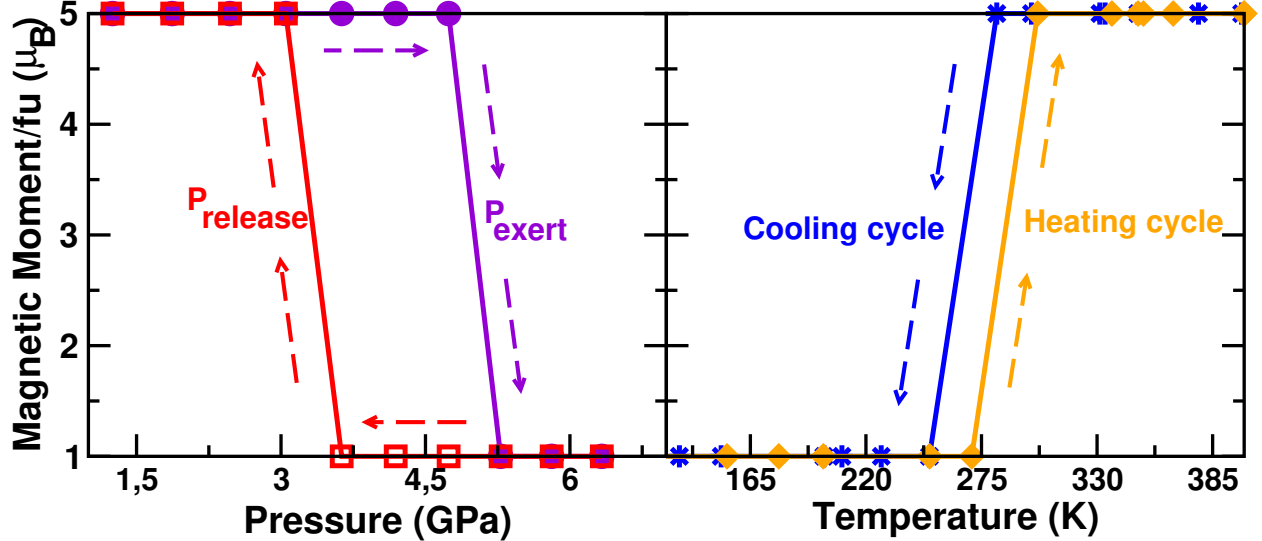
Figure 3: Pressure and temperature driven spin transitions accompanied by hystereses. The left panel shows the pressure-driven transition, whereas the right panel shows the temperature-driven transition obtained by a combination of MD simulations.
