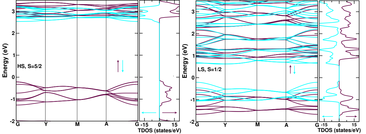
Figure 2: Figure showing the electronic structure of DMAMnF in HS and LS states. The left panel shows the spin-resolved band structure and DOS for the HS state, whereas the right panel shows the spin-resolved band structure and DOS for the LS state.
