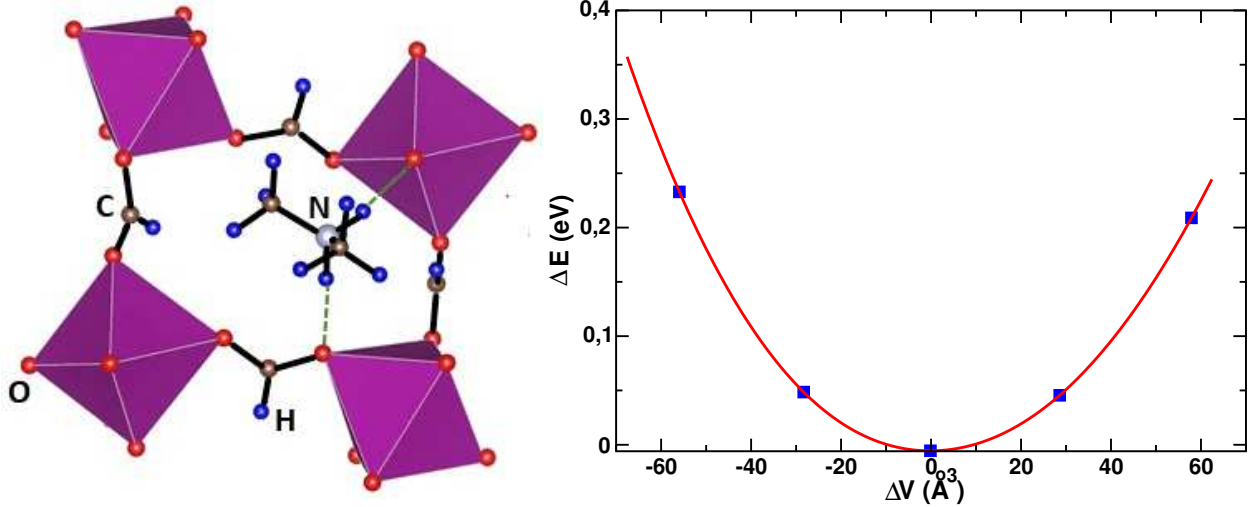
Figure 1: Structural details of DMAMnF. The left panel shows an image of the structure. The violet octahedra are the \text{MnO}_6 octahedra, with Mn being the B cation, connected by formate bridges forming the X anions, and the DMA cation sits in the cavity forming the A cation in the hybrid perovskite. The possible H bonds are marked by green dashed lines. The right panel shows a Birch-Murnaghan fit to obtain the bulk modulus of the material.
