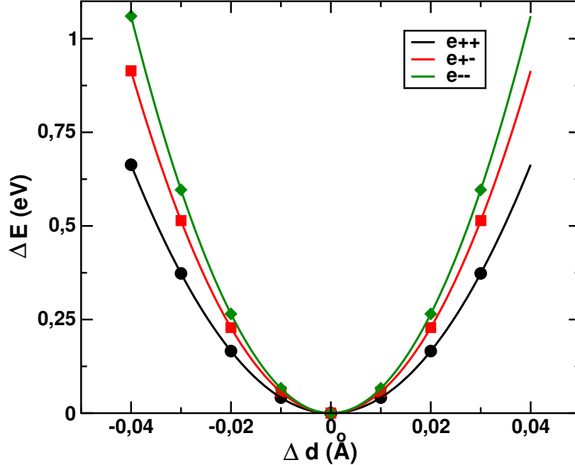
Figure 5: The figure shows the fit of the plots of Change in energy to change in bond-length to calculate the elastic constants.
