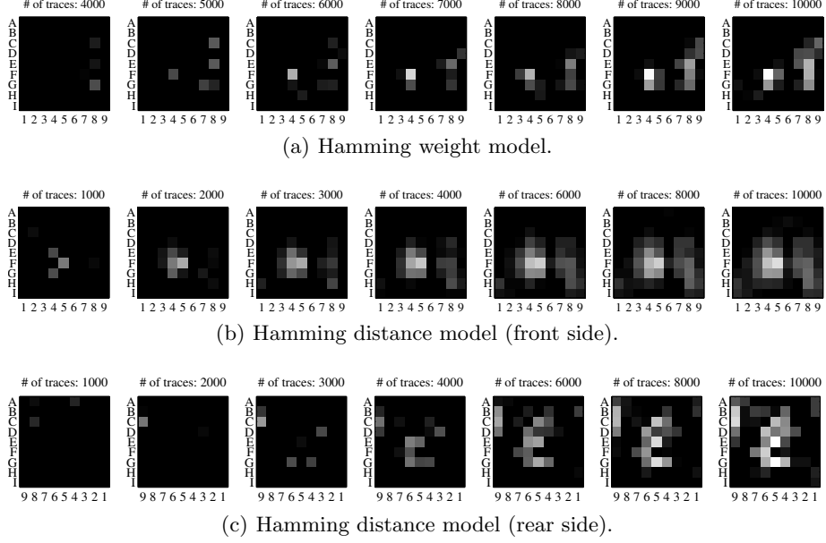
Fig. 7. EM-leakage landscape for different numbers of traces used for the CEMA attacks on the AES crypto engine. Note that for (a) and (b) the covered area is 9 x 9 mm, while for (c) the covered area equals 5 x 5 mm.
