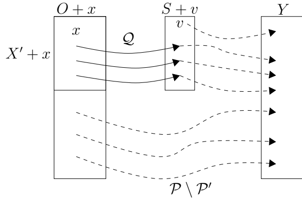
FIGURE 4.1. The construction of a path-system that joins O to Y in D - v .
