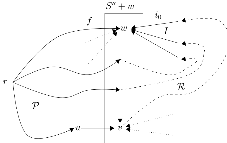
FIGURE 4.2. The separator S'' + w and path-system \mathcal{P} .
