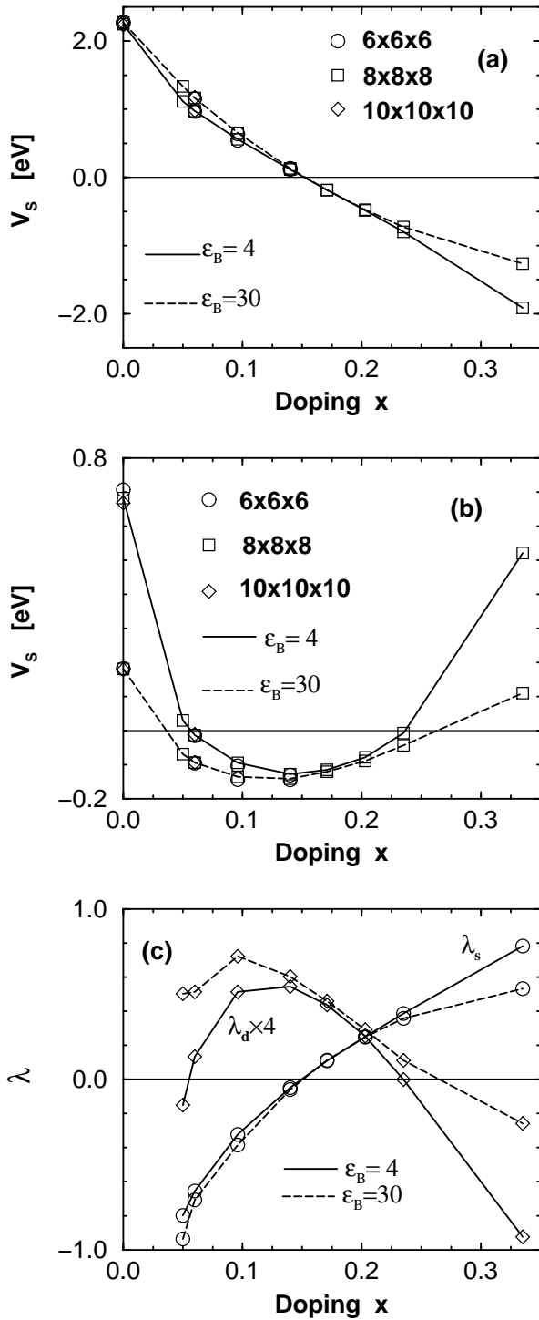
FIG. 1. Screened Coulomb potential V_S(r) \equiv V_S(r, i\omega = 0) at (a) on site ( r = 0 ) and (b) at in-plane 1st neighbor lattice vectors r and (c) Eliashberg \lambda -parameters for in-plane 1st neighbor d_{x^2-y^2} and on-site/1st neighbor s -wave pairing, all plotted vs. hole doping concentration x = 1 - \langle n_j \rangle at \beta t \equiv t/T = 3.0 and \Delta\tau t = 0.0375 for \epsilon_B = 4 and 30. In (a) and (b), results are for La_2CuO_4 with bct lattice sizes 6 \times 6 \times 6 , 8 \times 8 \times 8 and 10 \times 10 \times 10 , with estimated statistical uncertainties in V_S of less than 0.01eV. In (c), results are based on 8 \times 8 \times 8 data for V_S . \lambda_d is scaled \times 4 for display.
