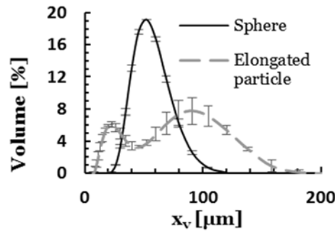
Figure 1: Evaluation of Mastersizer 200 with elongated and spherical test particles
