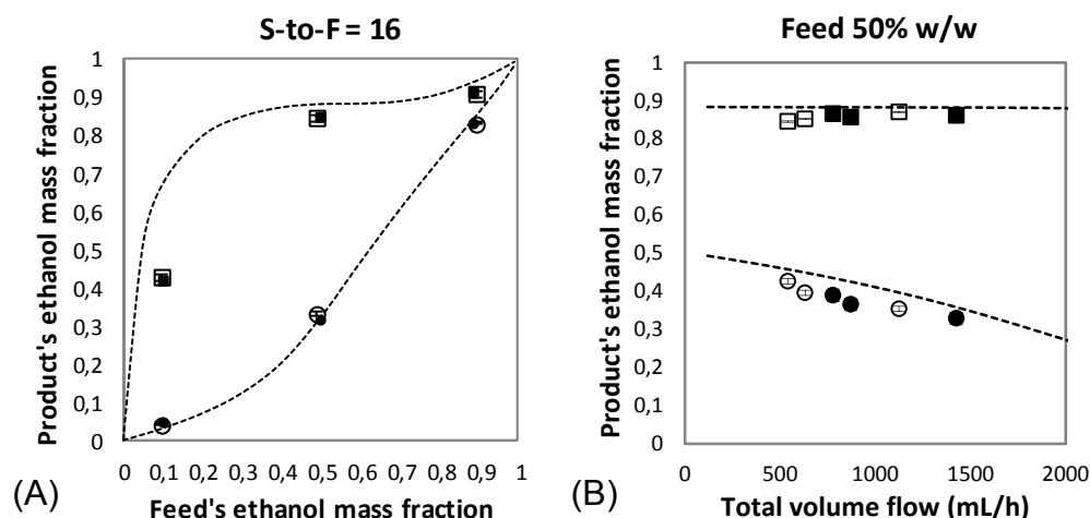
Figure 2. On the left side (A), comparison of experimental results of raffinate and extract compositions using the multi-lamination micro-mixer (●, ■) and the Tee-mixer (○, □) with the model result of one single theoretical stage ( S\text{-to-}F = 16 ). On the right side (B), product's ethanol mass fraction, raffinate (●, ○) and extract (■, □), as a function of the total volume flowrate in the micro-device (constant feed volume flowrate of 30 mL/h, variable \text{CO}_2 volume flowrate) for a feed composition of 50% w/w.
