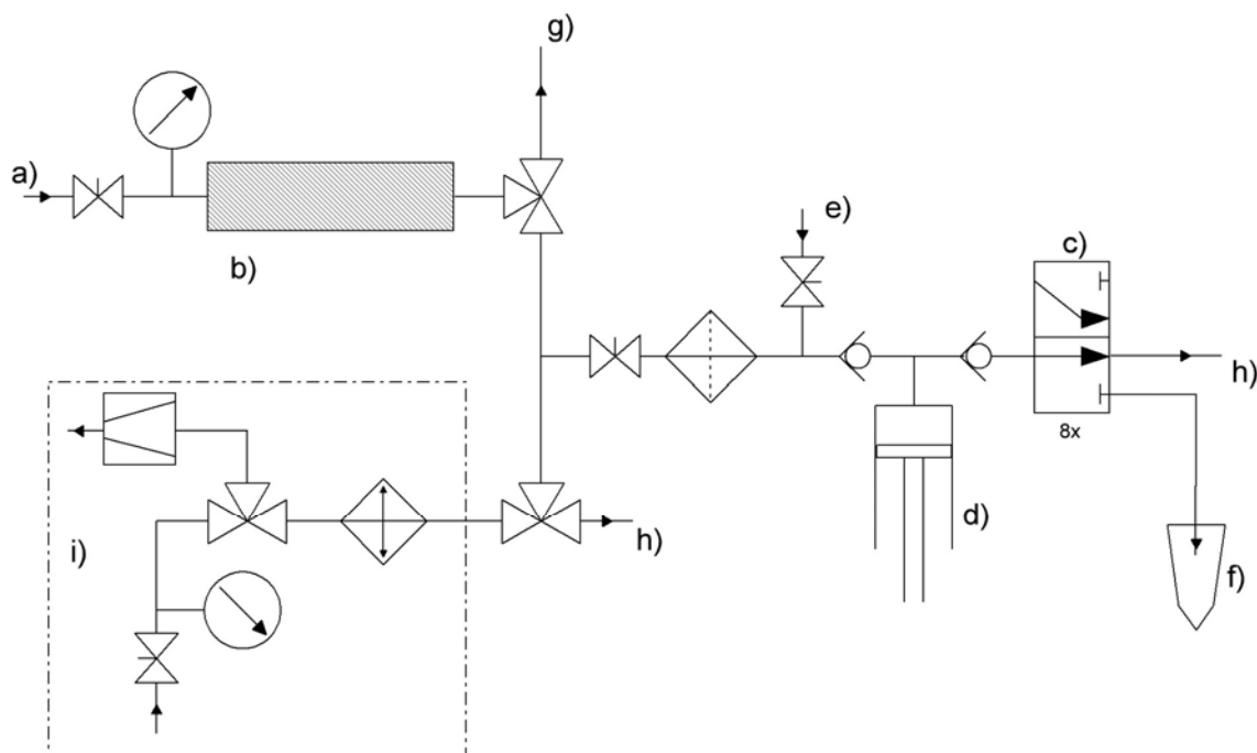
Fig. 1: Thermal runaway test rig consisting of a) carrier gas inlet ( N_2 ), b) tubular reactor with sample, c) multi-port valve, d) syringe pump, e) vial purge gas (Ar), f) crimp vials, g) optional impinge system, h) off gas and i) optional multi-purpose vacuum system.
