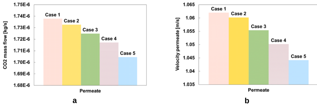
Figure 5: \text{CO}_2 mass flow and outlet velocities at permeate outlet for different cases
