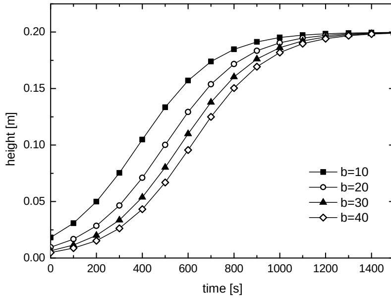
Fig. 2: Effect of parameter b (equation 1) on the induction period ( h_{\max} = 0.2 m, c = 0.006 ).
