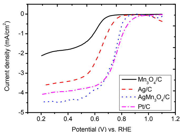
Fig. 3. Linear potential scan curves of Pt/C, Ag/C, \text{Mn}_3\text{O}_4/\text{C} and \text{AgMn}_3\text{O}_4/\text{C} electrocatalysts on a rotating disk electrode in an \text{O}_2 saturated 0.1 M KOH at 30 °C, with a sweep rate of 10 \text{ mV s}^{-1} and a rotation rate of 1600 rpm.
