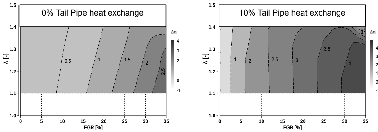
Illustration 2: \Delta\eta = f(\text{EGR}, \lambda)
