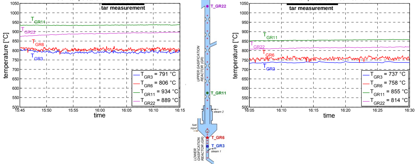
Figure 2: Temperature trend of GR for fuel SCB and EOP.
