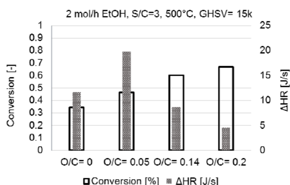
Illustration 5: Conversion and \Delta H_R vs. O/C
