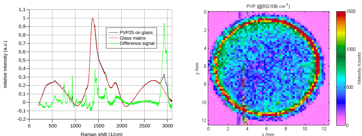
Figure 3: Left panel: Raman spectra of PVP solution on glass substrate. Right panel: Raman map of a PVP coated tablet. Specific-selected intensity plot in the wave number range of 932 to 936 cm -1 depicts the distribution of key component PVP.
