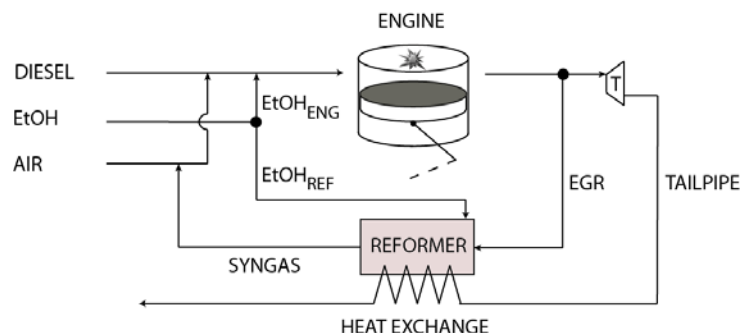
Illustration 1: TCR System
