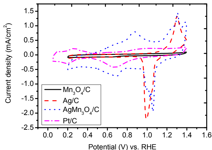
Fig. 2. Base cyclic voltammograms of Ag/C, \text{Mn}_3\text{O}_4/\text{C} and \text{AgMn}_3\text{O}_4/\text{C} electrocatalysts in a deaerated 0.1 M KOH at 30 °C, with sweep rate of 10 \text{ mV s}^{-1} .
