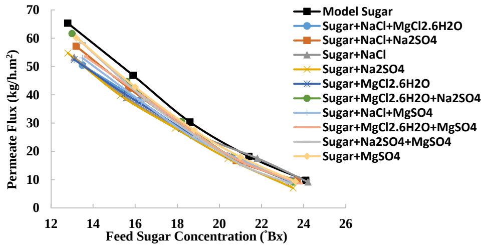
Fig 1. Influence of the sugar concentration on the permeate flux
