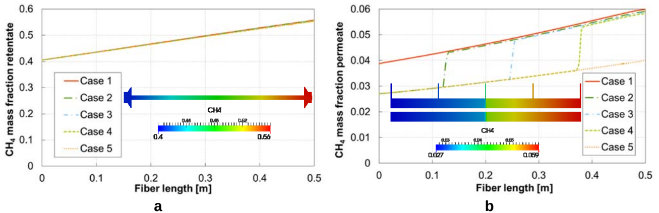
Figure 4: \text{CH}_4 mass fraction profiles and contour (case 3) for fiber and shell side
