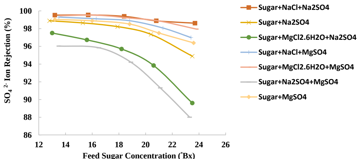
Fig 6. Rejection of \text{SO}_4^{2-} ion as a function of feed sugar concentration
