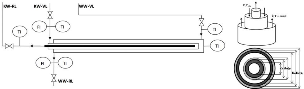
Figure 1: Set-up of the empirical measurements and a cross-section of the CBHE of the numerical model.
