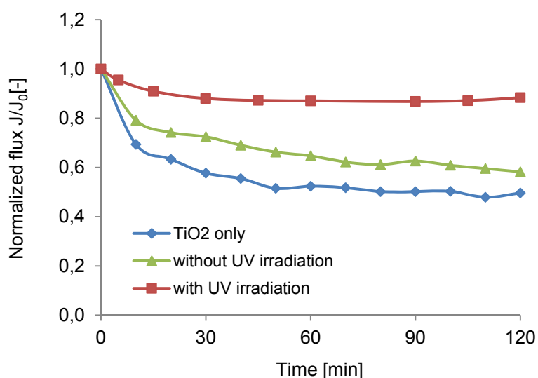
Figure 3: Variation of the normalized flux with different operating modes ( C_{TiO_2} = 0.5 g/L, Permeate flux J_p = 140 - 144 L/m²h)
