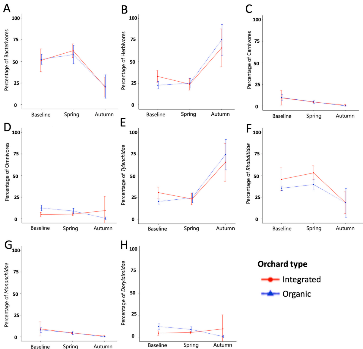
Fig. 4. Line graphs showing the average percentage proportion of nematode trophic guilds (a, b, c, and d), and family (e, f, g, and h) dynamics between baseline, spring, and autumn, respectively. The line graphs are based on n = 4 samples at each sampling time, both for organic, and integrated fields sampled. The different nematode families are categorized into the trophic guilds: Tylenchidae (herbivores), Rhabditidae (bacterivore), as well as Dorylaimidae and Mononchidae (omnivores and carnivores).
