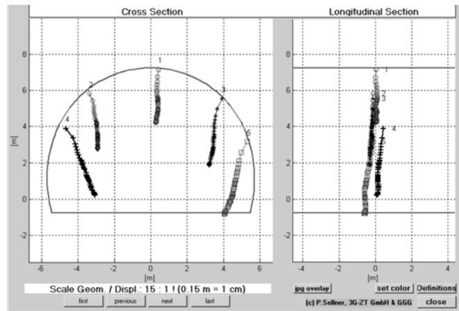
Fig. 8. Measured displacements for example 3.
