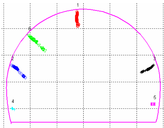
Figure 1. The displacement vector orientation in cross section
