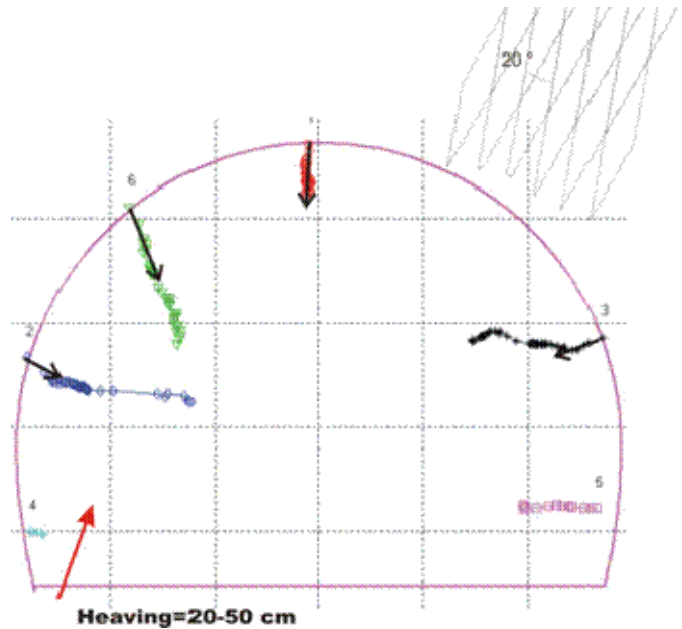
Figure 2. Measured and calculated displacement vectors at the cross section (1935m)
