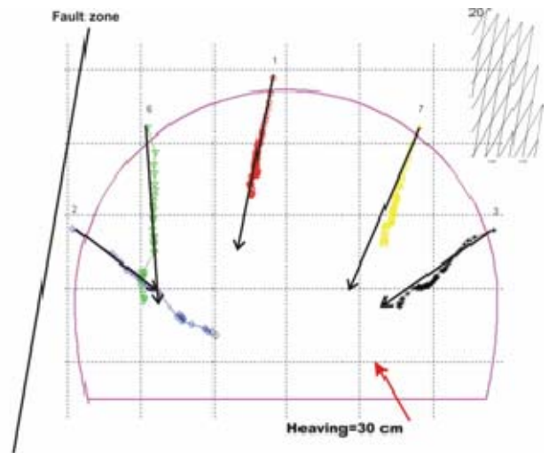
Figure 7. Measured and calculated displacements and their vectors at the cross section (2188m) considering a fault zone outside the tunnel cross section.
