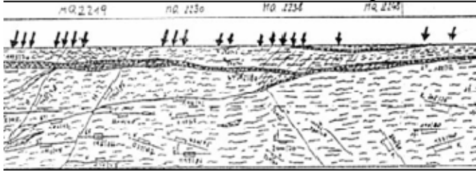
Figure 9. Geological plan view
