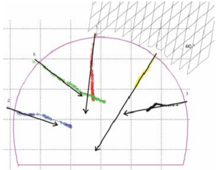
Figure 11. Measured and calculated displacements and their vectors at the cross section (2306m)
