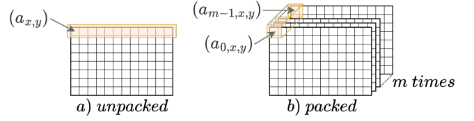
Figure 2: Overview of packed and unpacked memory format
